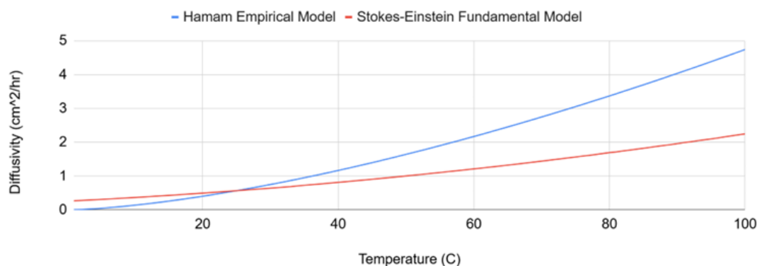
Figure 1: Diffusivity Versus Temperature for Crude Oil in Water According to Two Different Models.
