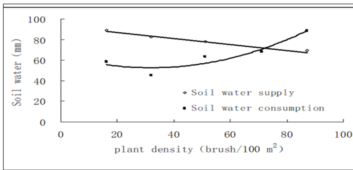
Fig.1 The change of soil water supply or consumption with plant density in the critical period of plant-water relationship regulation in Caragana shrubland (Guyuan, China)
