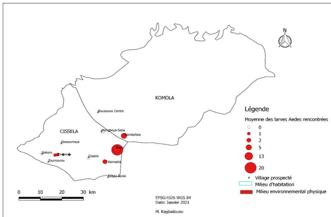
Figure 7: Distribution of potential breeding sites and average numbers of Aedes larvae encountered in Kouroussa from January 16 to 20, 2021
